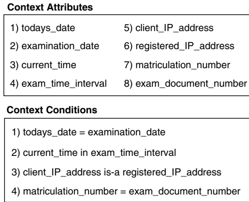
Figure 5: Context attributes and conditions
