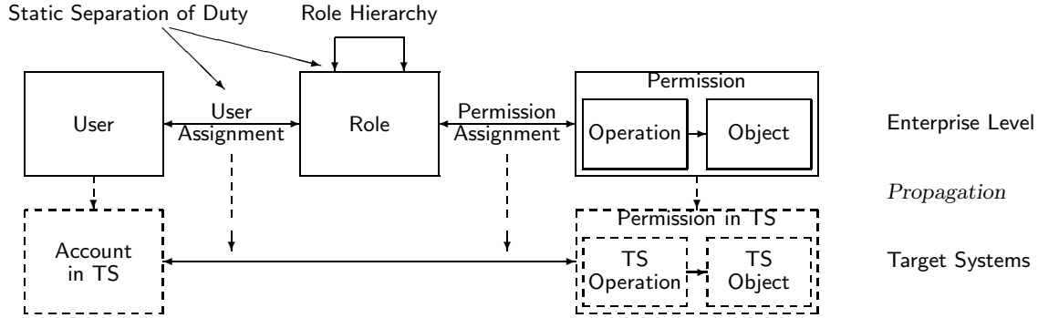
Figure 2: Enterprise RBAC Model (ERBAC)
